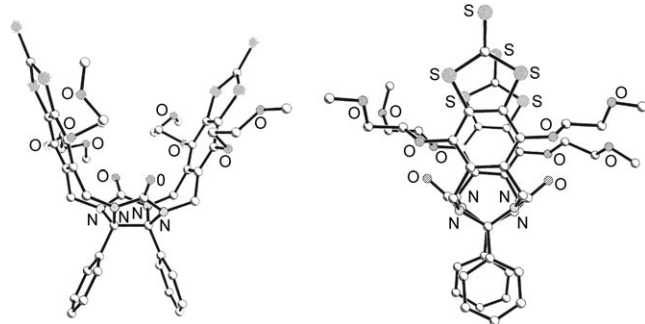
Figure 4. Ball-and-stick representations of the solid-state structure of molecular clip 5c .
