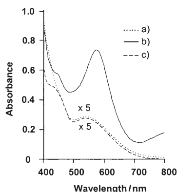
Figure 9. Partial UV-visible spectra (MeCN, 298 K) of a) a mixture of 16 \cdot 2PF_6 and 1a (1 mm each), b) the mixture obtained after addition ( p -BrPh) 3 NSbCl 6 (1 equiv) to the solution in (a), and c) the mixture obtained after the addition of excess zinc powder to the solution in (b).
