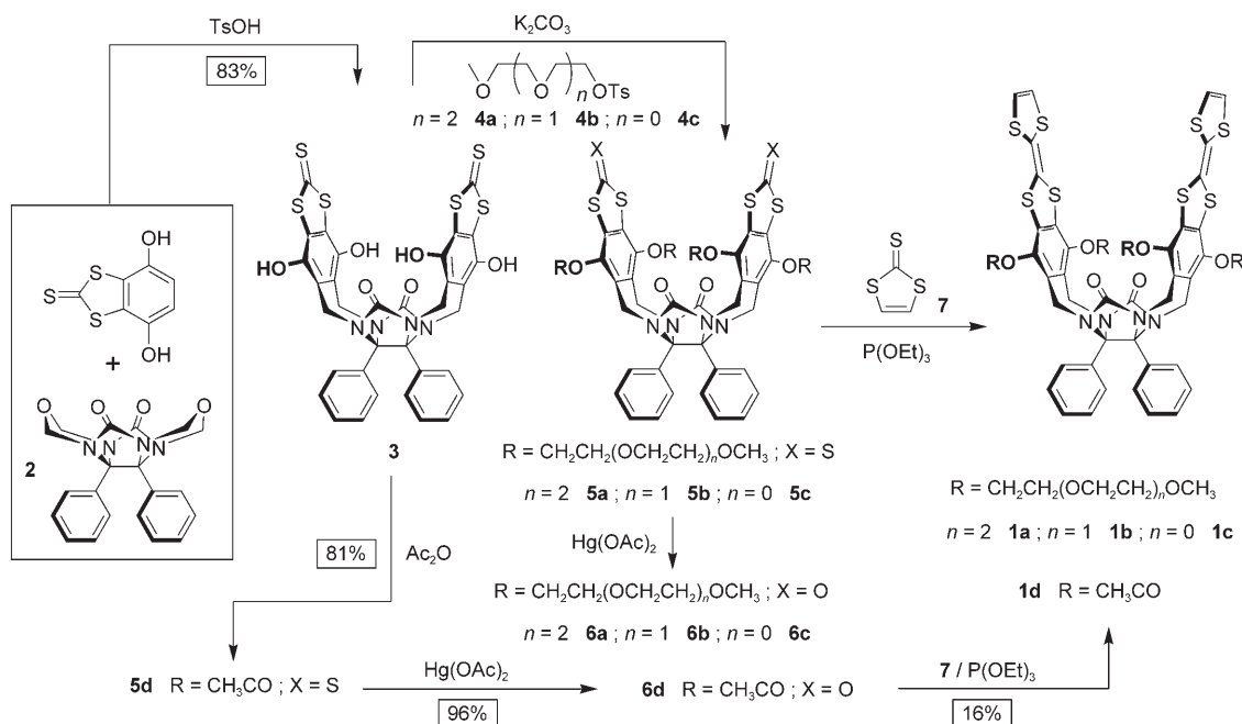
Scheme 1. Syntheses of the molecular clips 1a–d .
