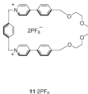
Scheme 5. Formation of the complex ( 11 ⊂ 1a )·2PF 6 .
