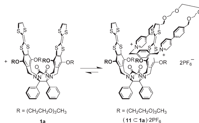
Scheme 5. Formation of the complex ( 11 ⊂ 1a )·2PF 6 .
