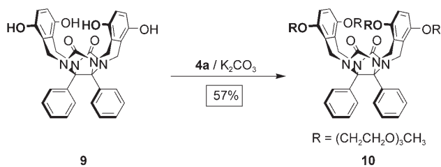
Scheme 3. Synthesis of molecular clip 10 .
